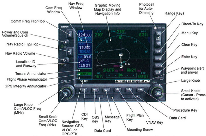
Figure 1 - 530W Series Control and Display Layout
